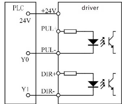
C PLC connection
