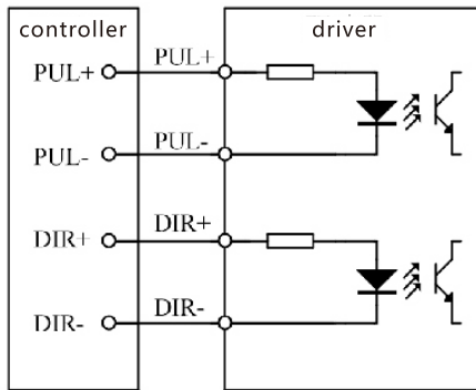
A 5V differential connection
