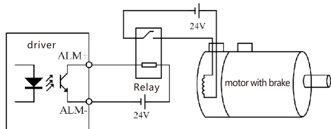
F Brake output connection
