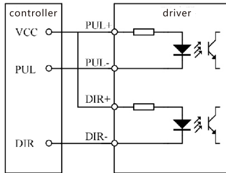
B 5V single-ended connection
