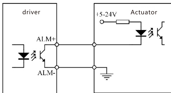
E Alarm output connection
